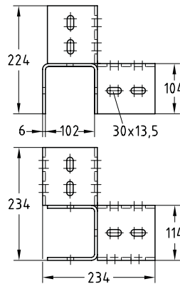
MPT-Corner connector
