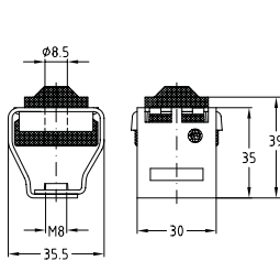
For M8
