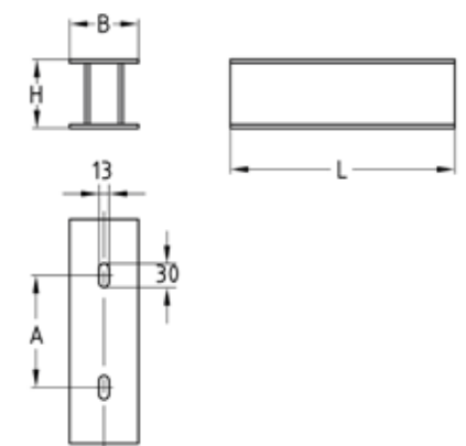
For profile Q80, Q150, schematic sketch (original may vary)
